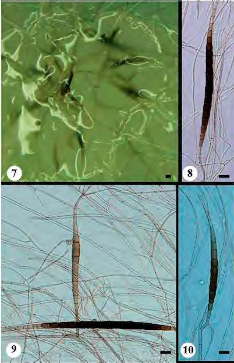
FIGS. 7–10. Xylomyces chlamydosporus produced from Jahmula aquatica ascospores. 7. Chlamydospores produced on CMA contaminated by bacteria. 8–10. Chlamydospores produced on CMA. Scale bars = 10 \mu\text{m} .
